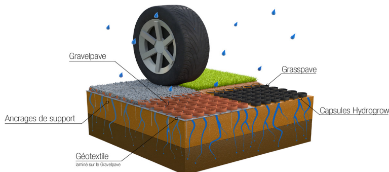
TEXEL GRASSPAVE / TEXEL GRAVELPAVE
