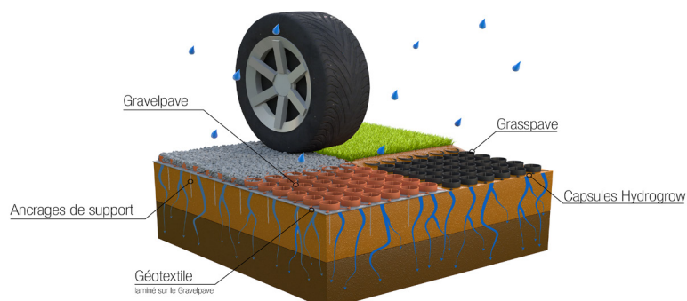
TEXEL GRASSPAVE / TEXEL GRAVELPAVE
